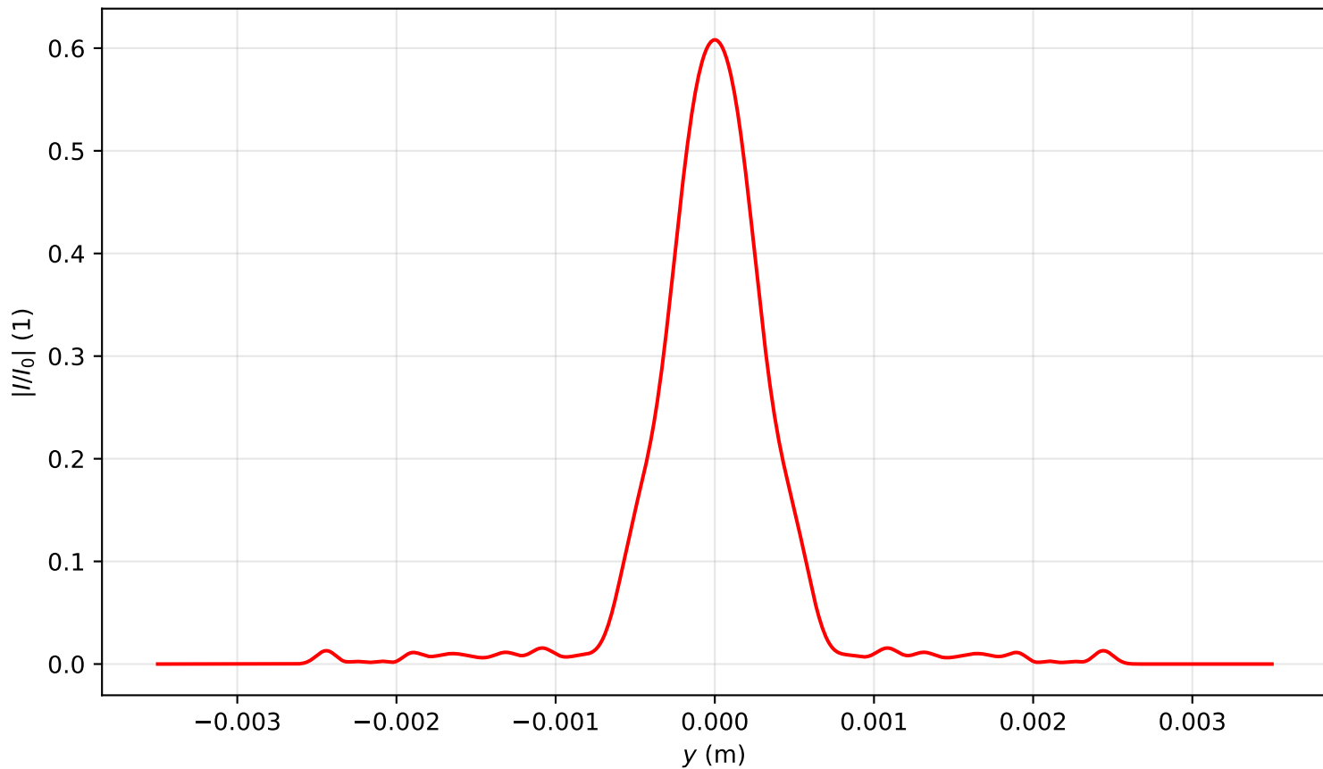
Intensity profile I(x=0, y, z=3.582)/I_0 , P_{in}=3.0P_{cr} , artificial time
